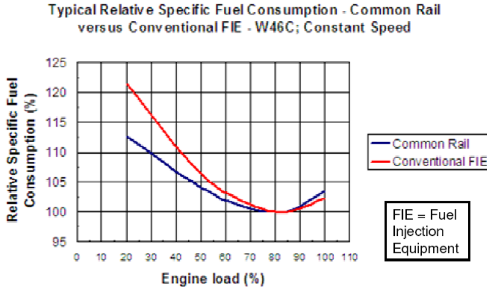
Figure 7.2: Relative Fuel Consumption of a Wartsila Engine at Different Loads
